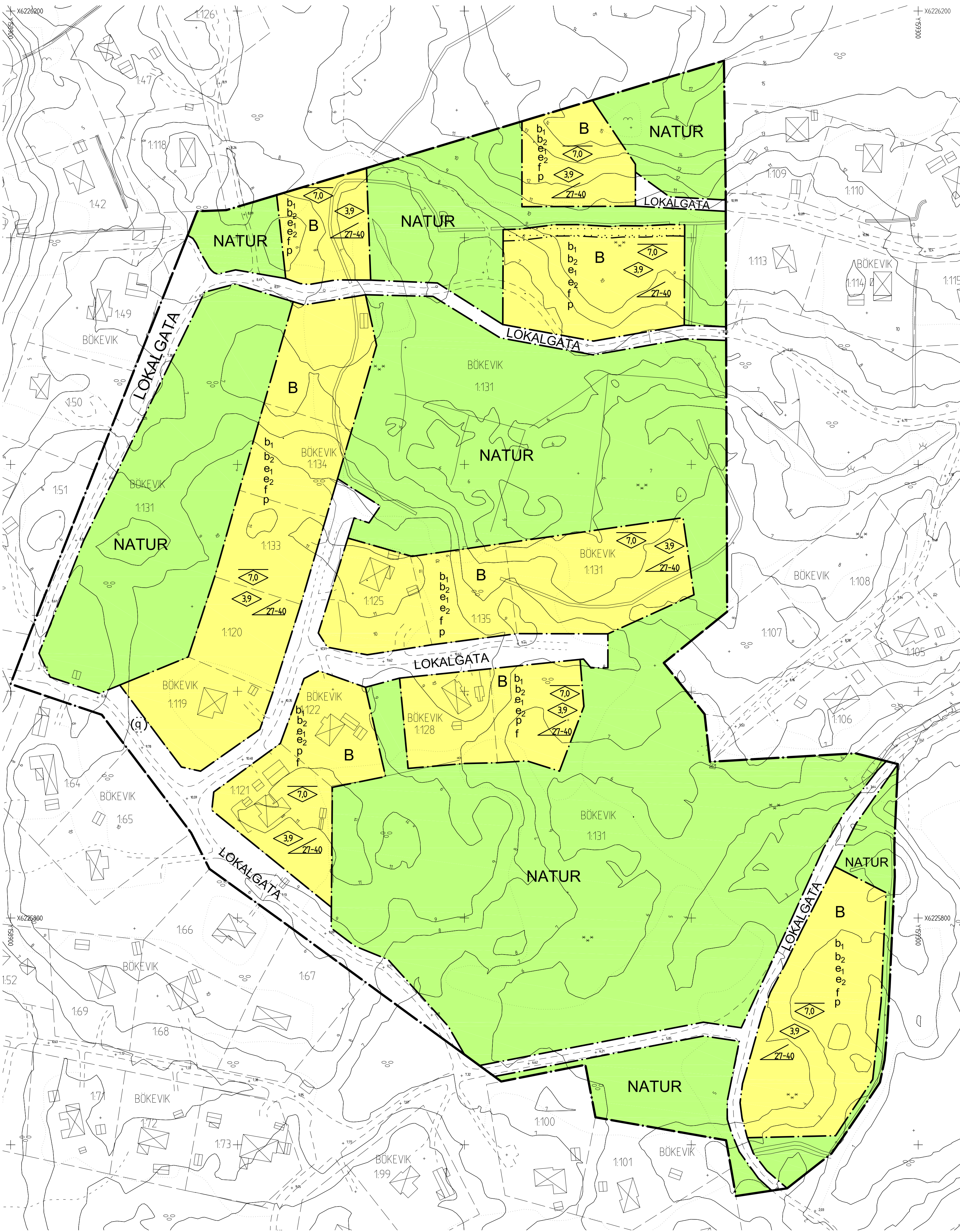
Plankarta 1:1000 (A1)
